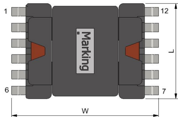
Part Outline
