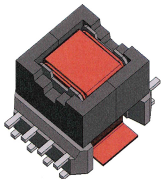
Part Outline
