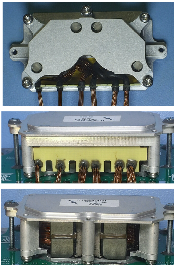
Part Mounting
