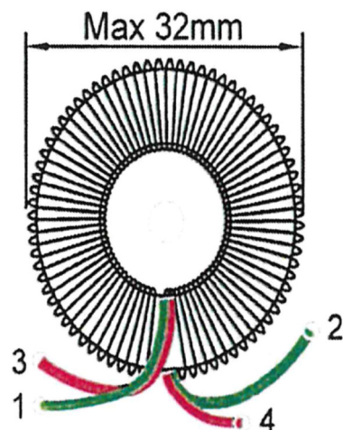
Part Outline
