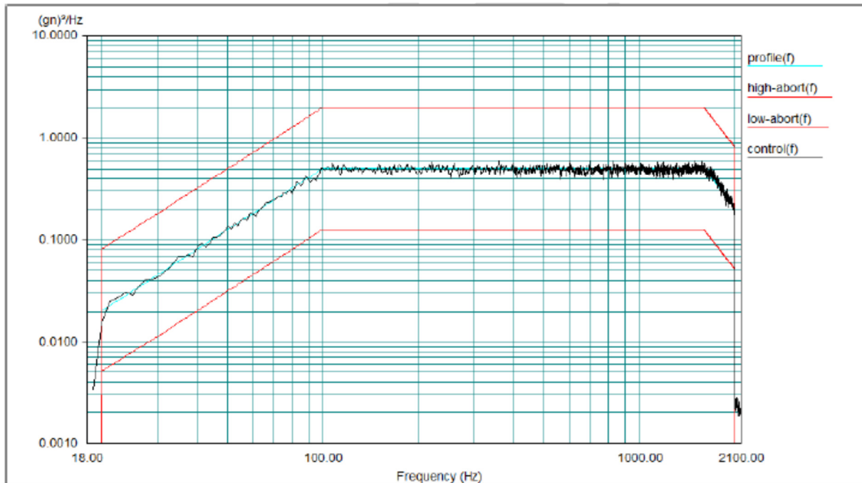
Curve 1 Exposure curve e.g. X-axis. Similar curve for all axes.
