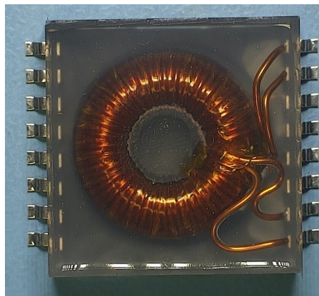
Part Mounting
